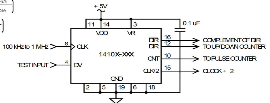
RECOMMENDED CONNECTIONS
