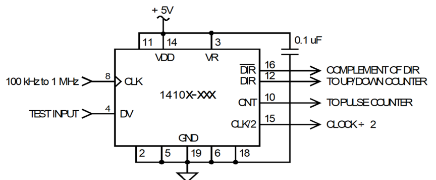
RECOMMENDED CONNECTIONS
